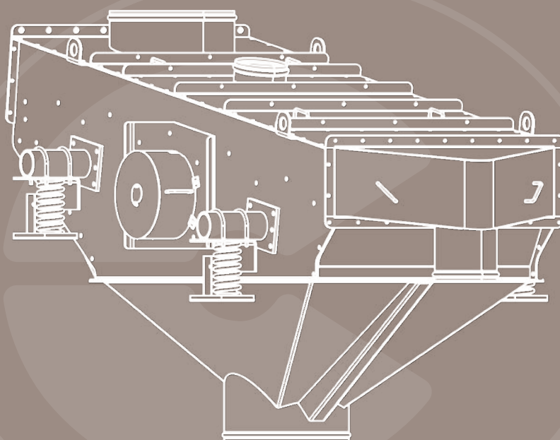
ROL HG with VIBRATING COVER & HOPPER
